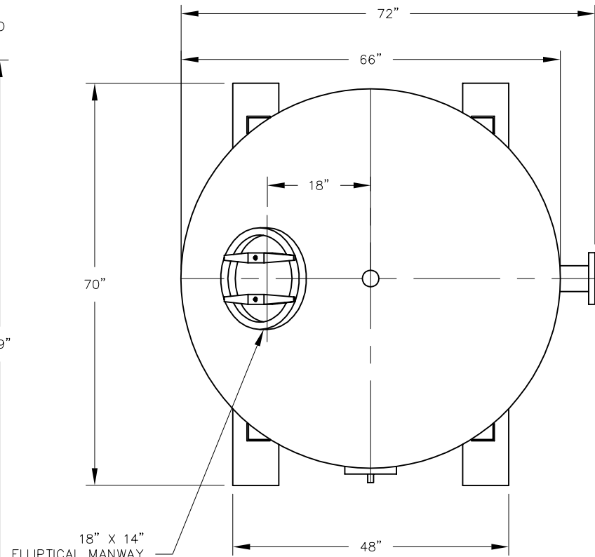
PLAN
